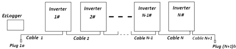
Fig3.4.2.3. Check the whole RS485 cable connection
